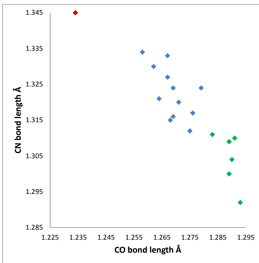
Figure 3. Comparison of C-N and C=O bond lengths (Å) for all known PAR and PAR(H) crystal structures. Red diamond = average values based on 66 well characterized neutral PAR species available in the CDS database. Green diamonds = cationic PAR(H) species. Blue diamonds = hemi-halides, the partially protonated species featuring H shared between hydrogen bonded PAR(H) and PAR moieties.
