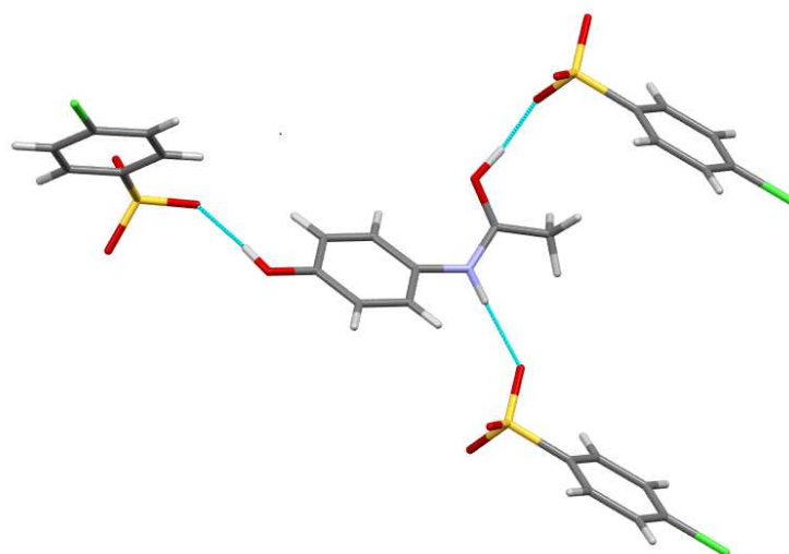
Figure 1. Part of the structure of [\text{PAR}(\text{H})][\text{SO}_3\text{C}_6\text{H}_4\text{Cl}] ( 1a ) showing that each cation forms three hydrogen bonds to three separate anions.
