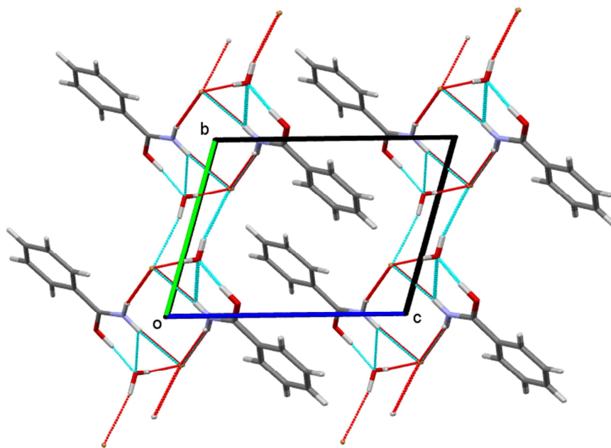
Figure 6. Packing diagram for structure ( 2a ) viewed along the crystallographic a direction. Note the formation of hydrophobic and hydrophilic layers.
