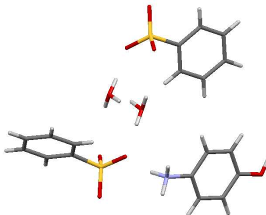
Figure 4. Asymmetric unit contents of [\text{H}_3\text{NC}_6\text{H}_4\text{OH}][\text{H}_3\text{O}][\text{O}_3\text{SC}_6\text{H}_5]_2 \cdot \text{H}_2\text{O} , ( 1d ). The proton positions situated between the water molecules each have a sof of 50%.
