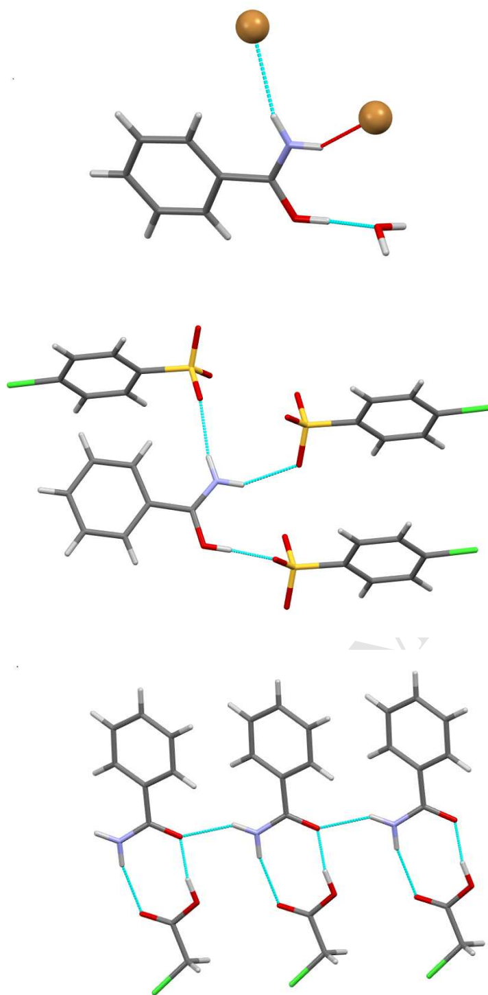
Figure 5. Each BEN(H) cation in salt forms [BEN(H)][Br].H 2 O ( 2a , top) and [BEN(H)][O 3 SC 6 H 4 Cl] ( 2b , middle) donates three hydrogen bonds to three neighbouring anions/molecules. However, the hydrogen bonding in the cocrystal BEN.HOOCCH 2 Cl ( 2c , bottom) is based on the classic amide/carboxylic acid R 2 2 (8) heterodimer.
