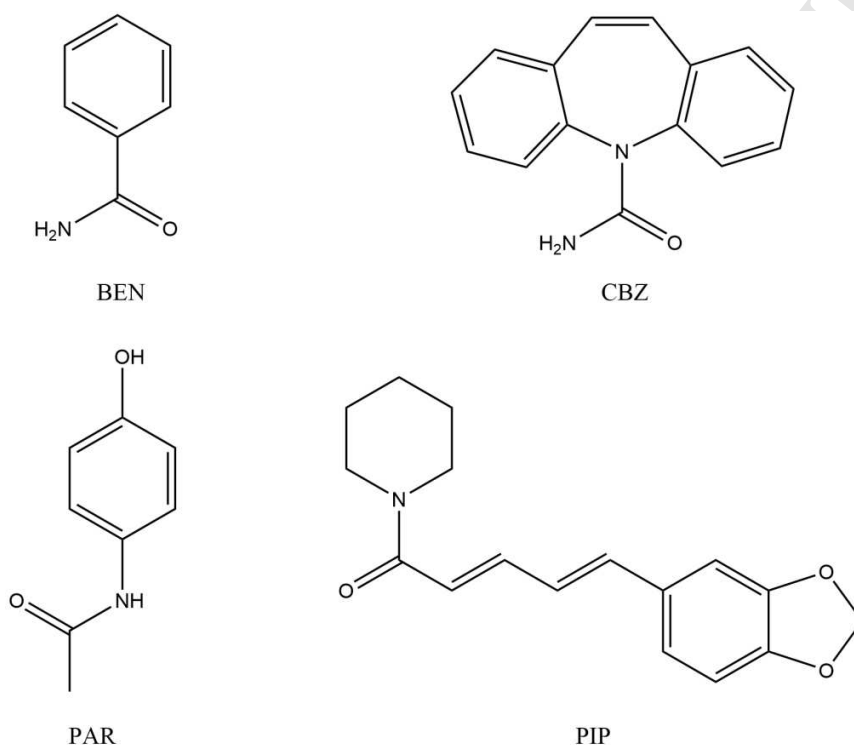
Scheme 1. Molecular structures of amides.
