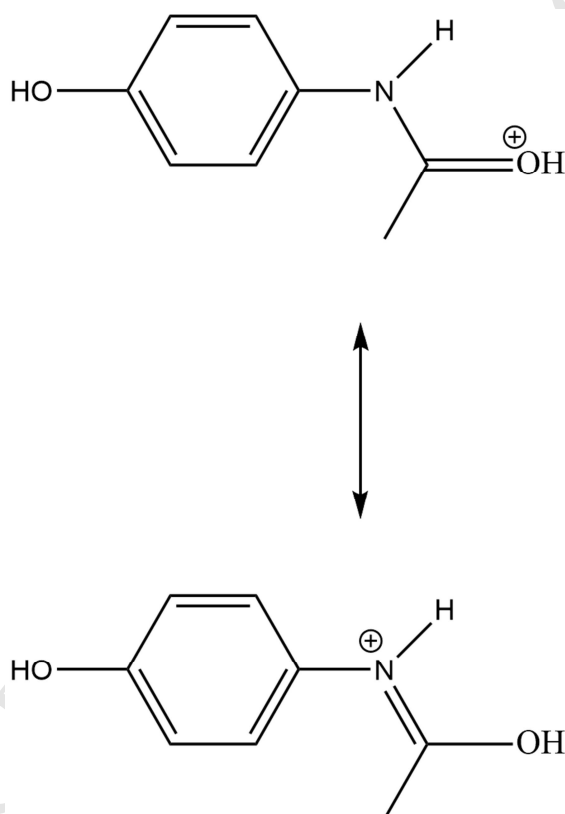
Scheme 2. Resonance forms of protonated paracetamol, PAR(H).
