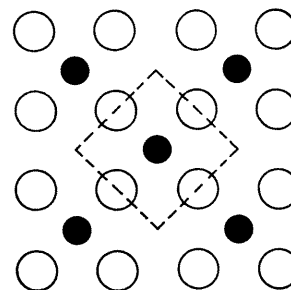
FIGURE. Suggested structure of silver ketenide (I) projected on to ab plane. Light circles denote silver atoms in plane of page (Ag–Ag = 2.84 Å, interplanar spacing 5.846 Å), and dark circles denote C-1 (of linear C 2 O groups) lying below this plane and eclipsing C-2 and O.
