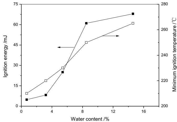
Fig. 7. Influence of water content on the ignition energy and minimum ignition temperature of sulfur dust.
