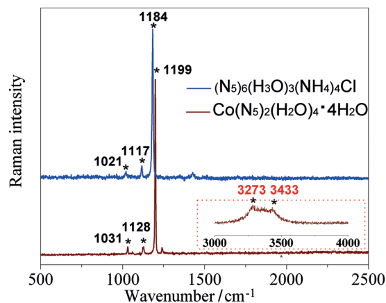
Figure 3. Raman spectra of \text{Co}(\text{N}_5)_2(\text{H}_2\text{O})_4\cdot 4\text{H}_2\text{O} and (\text{N}_5)_6(\text{H}_3\text{O})_3\text{-}(\text{NH}_4)_4\text{Cl} .
