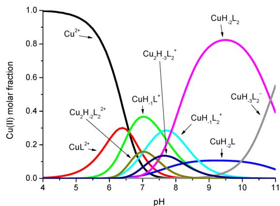
Figure 2. Species distribution of complexes calculated for 2.5 mM Tris and 1 mM Cu(II) on the basis of stability constants provided in Table 1, recorded at 25 °C and I = 0.1 (KNO 3 ).
