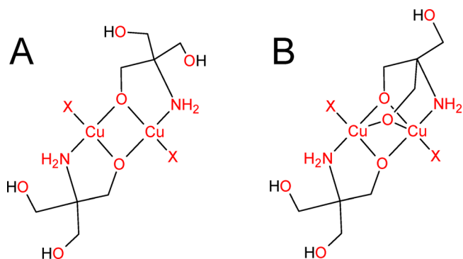
Figure 6. Probable structures of Cu 2 H -2 L 2 and Cu 2 H -3 L 2 dimers based on our experimental data and the published tetramer X-ray structure. 38 X represents a solvent molecule or a counterion.
