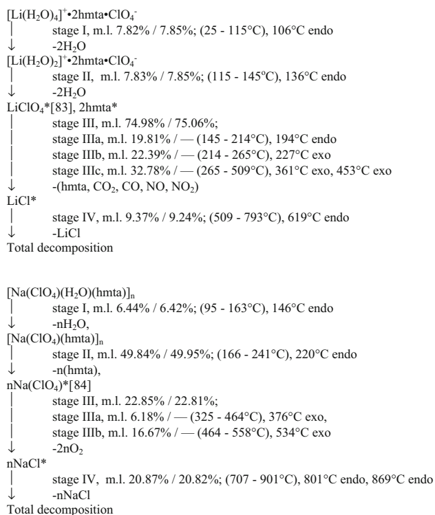
Scheme 2 The stages of thermal decomposition of the studied compounds (m.l.—experimental mass loss/theoretical mass loss, asterisk product confirmed by XRPD)
