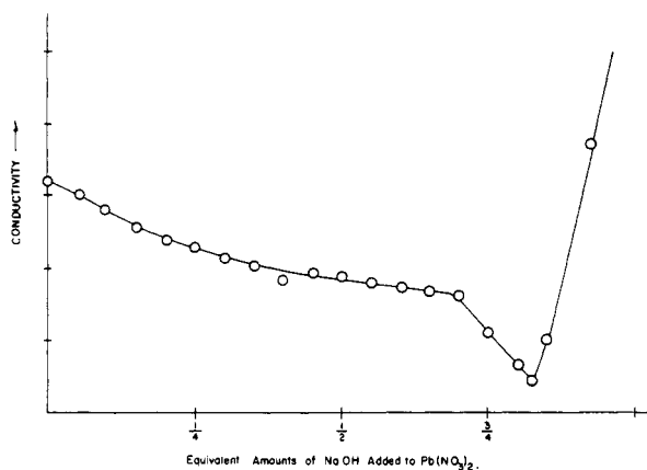
Fig. 1.—Conductometric titration of 0.1 N \text{Pb}(\text{NO}_3)_2 with 1 N \text{NaOH} , corrected conductivity expressed in arbitrary units.
