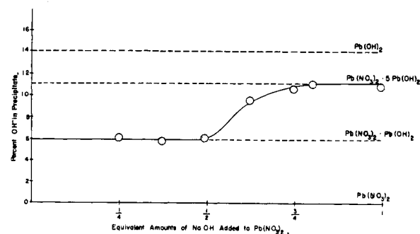
Fig. 3.—Variation in the composition of the precipitate formed by the titration of 0.1 N \text{Pb}(\text{NO}_3)_2 with 1 N \text{NaOH} expressed in terms of \text{OH} -analysis.
